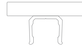
DRINK RAIL SELECT FROM ANY FULL PROFILE, SQUARE-SHOULDER DECK BOARDS. NOT COMPATIBLE WITH GROOVED OR SCALLOPED BOARDS.
